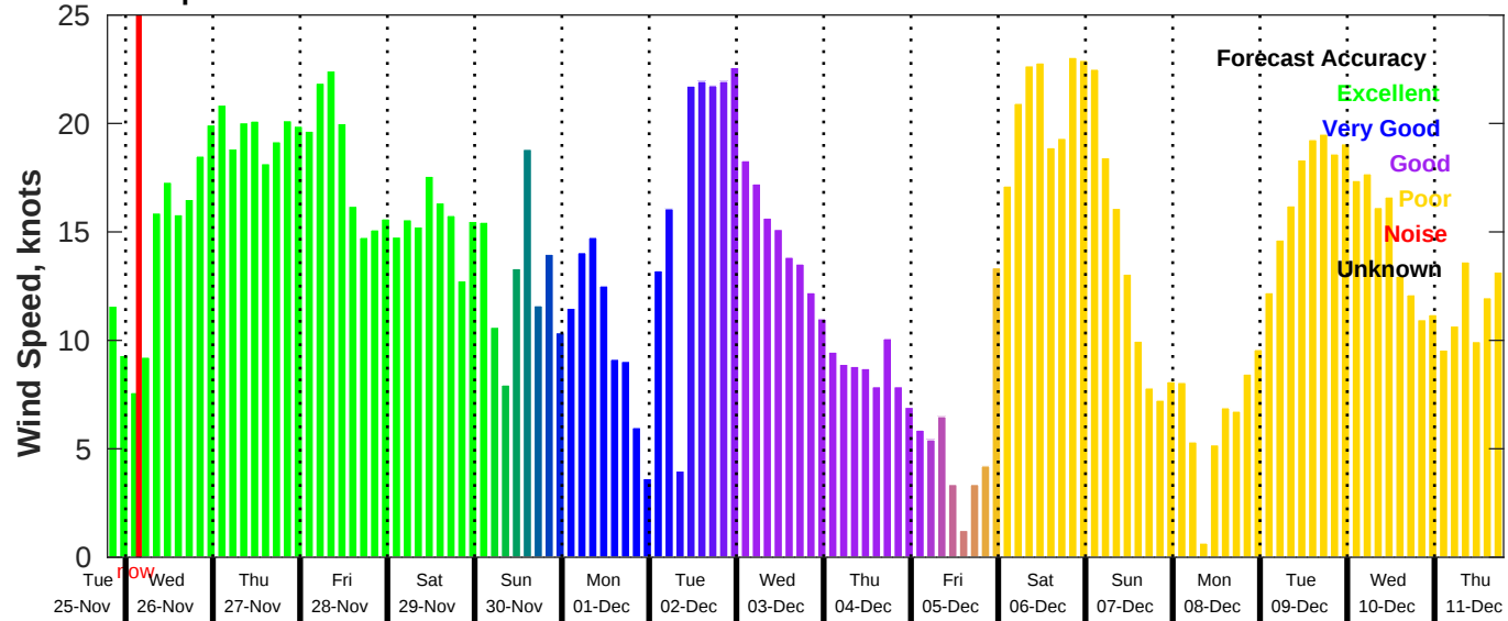
GFS Wind Speed Forecast for NDBC 42040 from 25-Nov-2025 19:00:00 to 11-Dec-2025 19:00:00
