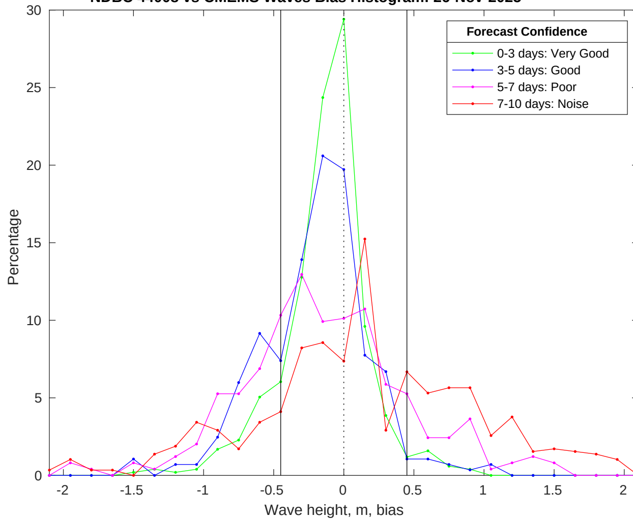
NDBC 44008 vs CMEMS Waves Bias Histogram: 26-Nov-2025
