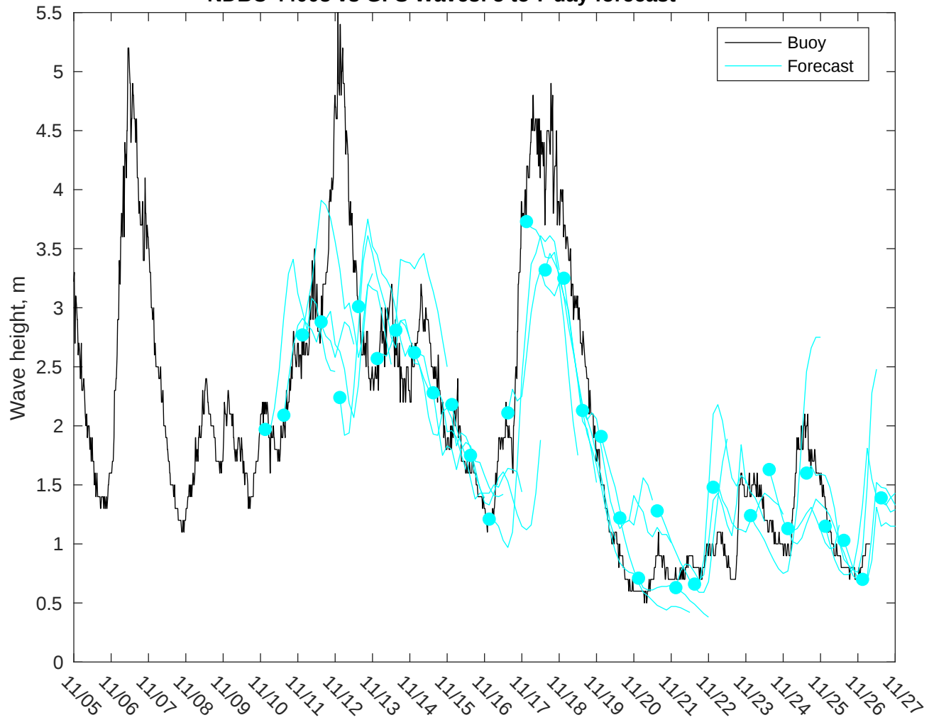
NDBC 44008 vs GFS Waves: 5 to 7 day forecast
