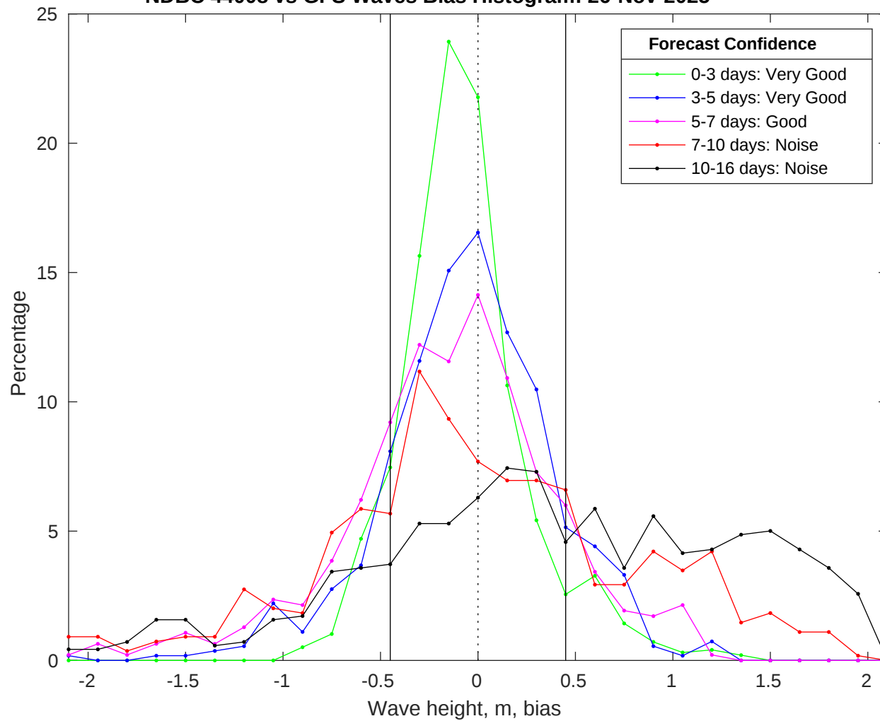
NDBC 44008 vs GFS Waves Bias Histogram: 26-Nov-2025
