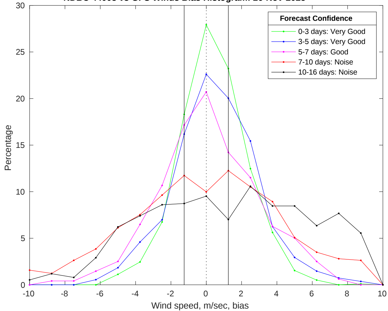
NDBC 44008 vs GFS Winds Bias Histogram: 26-Nov-2025
