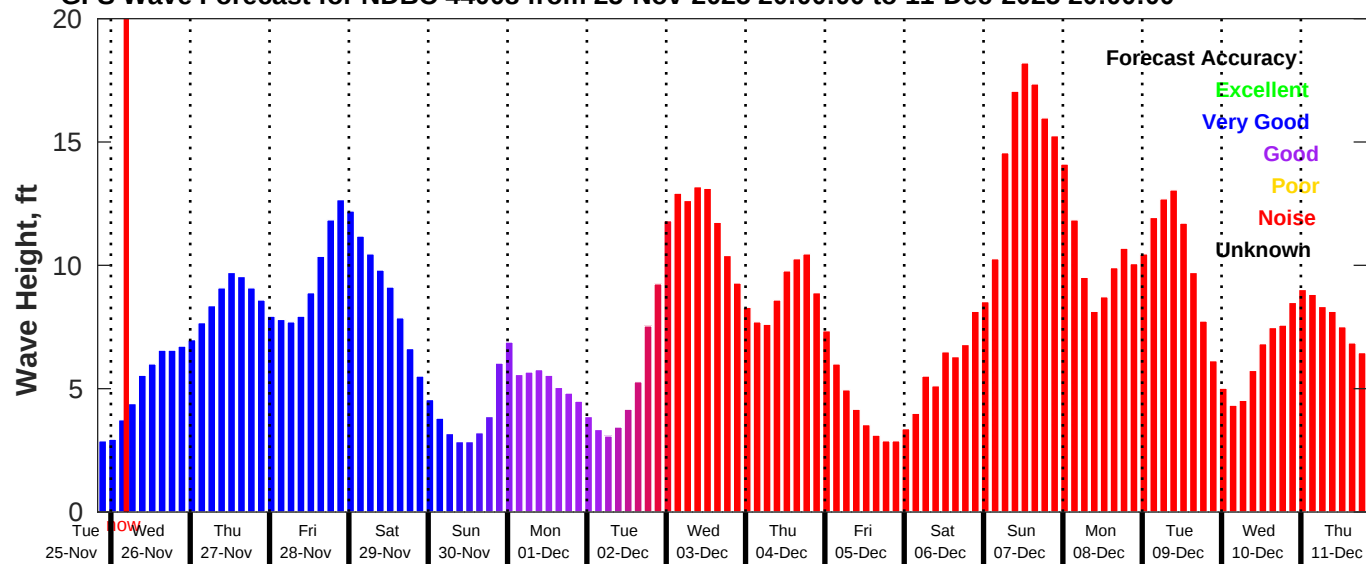
GFS Wave Forecast for NDBC 44008 from 25-Nov-2025 20:00:00 to 11-Dec-2025 20:00:00
