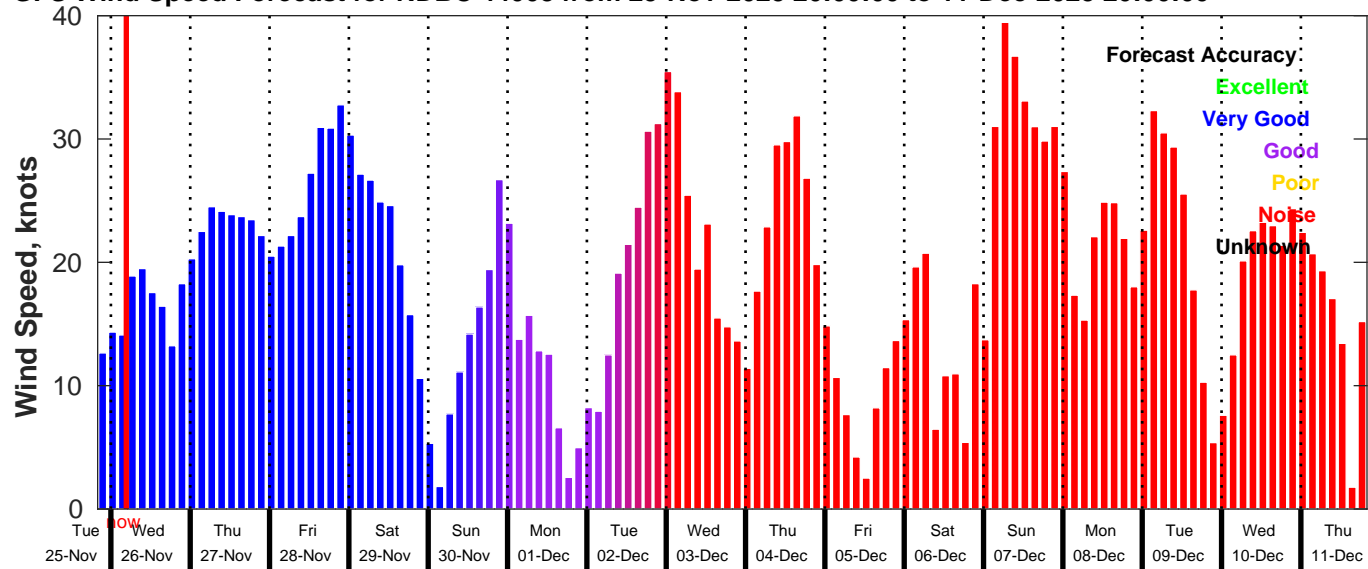
GFS Wind Speed Forecast for NDBC 44008 from 25-Nov-2025 20:00:00 to 11-Dec-2025 20:00:00
