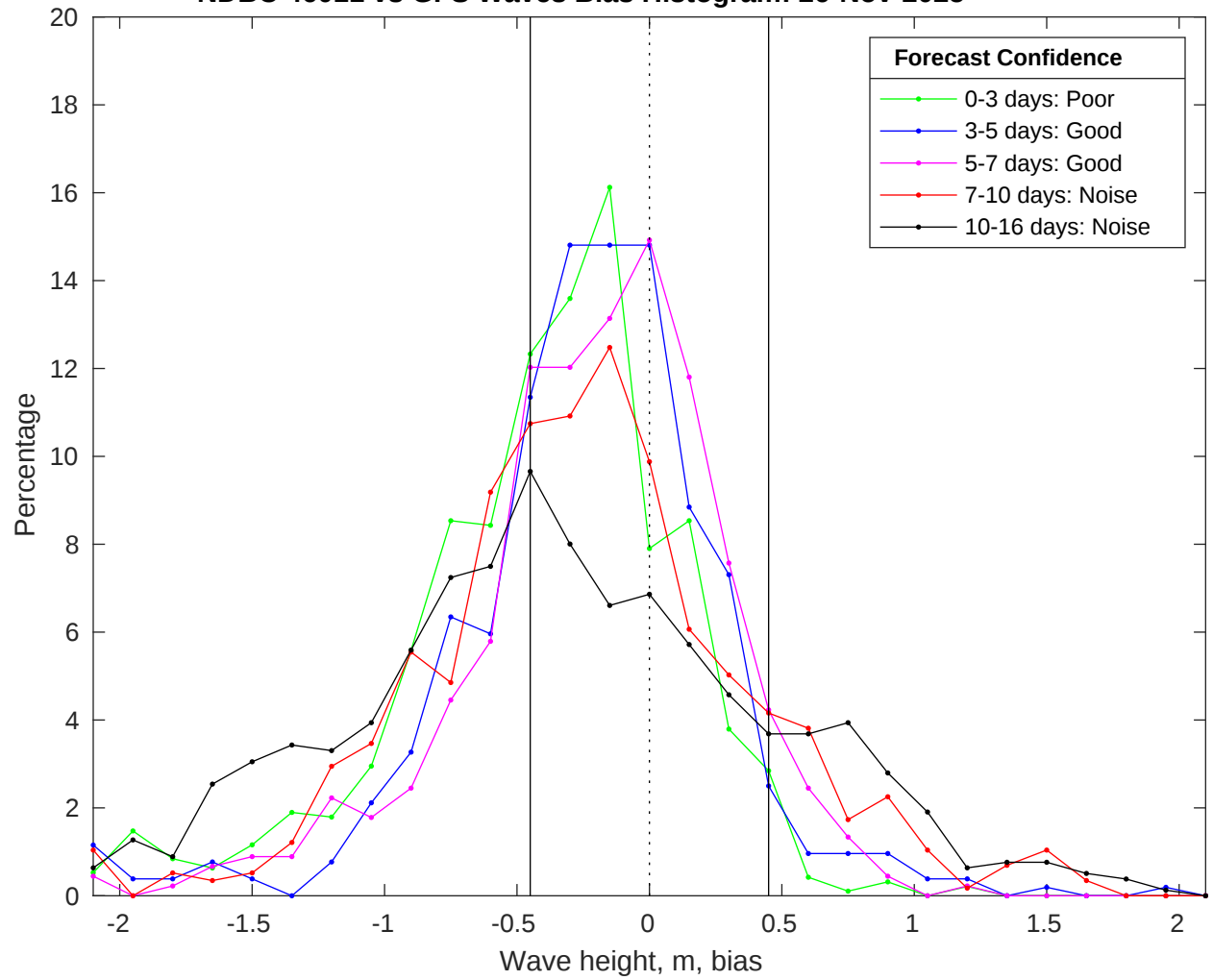
NDBC 46011 vs GFS Waves Bias Histogram: 26-Nov-2025
