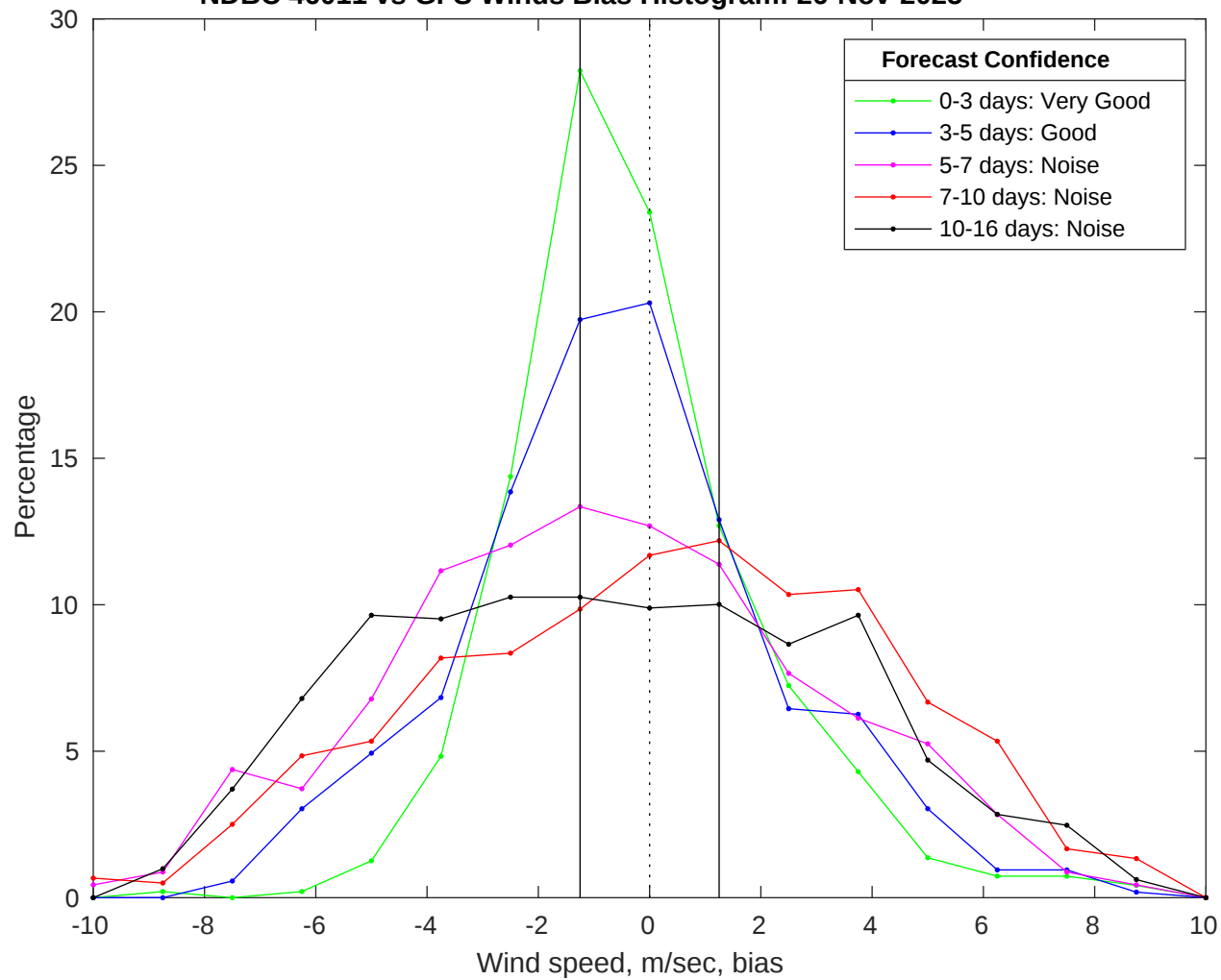
NDBC 46011 vs GFS Winds Bias Histogram: 26-Nov-2025
