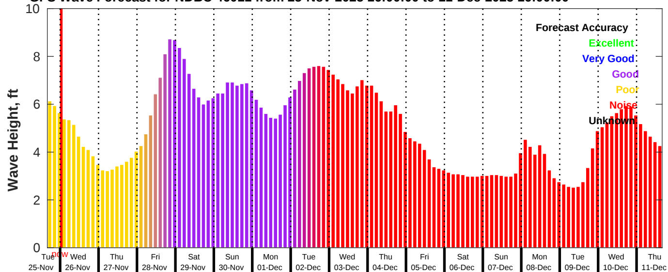
GFS Wave Forecast for NDBC 46011 from 25-Nov-2025 16:00:00 to 11-Dec-2025 16:00:00
