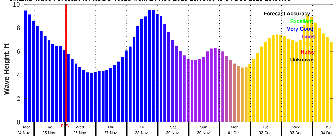
CMEMS Wave Forecast for NDBC 46028 from 24-Nov-2025 16:00:00 to 04-Dec-2025 16:00:00
