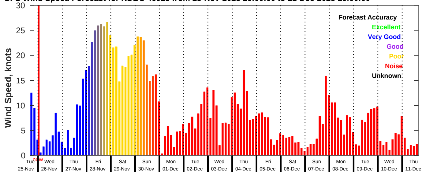
GFS Wind Speed Forecast for NDBC 46028 from 25-Nov-2025 16:00:00 to 11-Dec-2025 16:00:00
