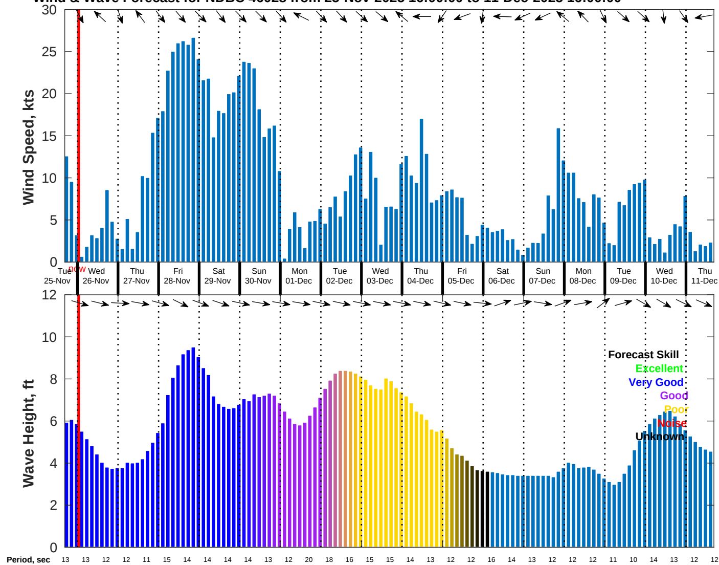
Wind & Wave Forecast for NDBC 46028 from 25-Nov-2025 16:00:00 to 11-Dec-2025 16:00:00
