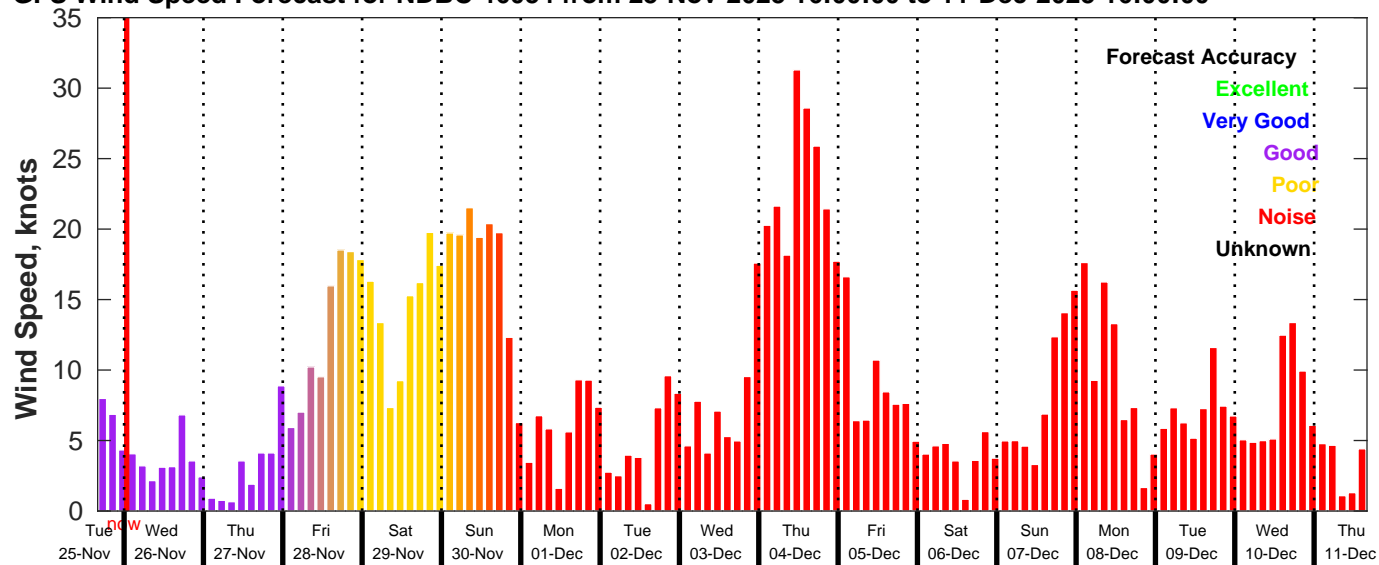
GFS Wind Speed Forecast for NDBC 46054 from 25-Nov-2025 16:00:00 to 11-Dec-2025 16:00:00
