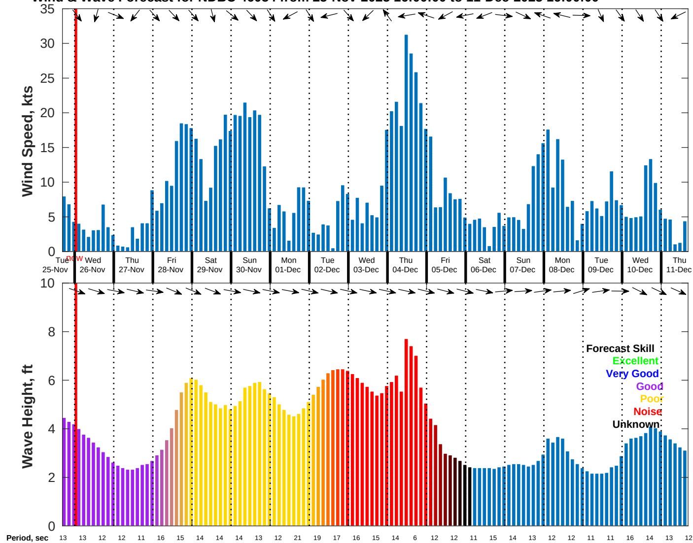
Wind & Wave Forecast for NDBC 46054 from 25-Nov-2025 16:00:00 to 11-Dec-2025 16:00:00
