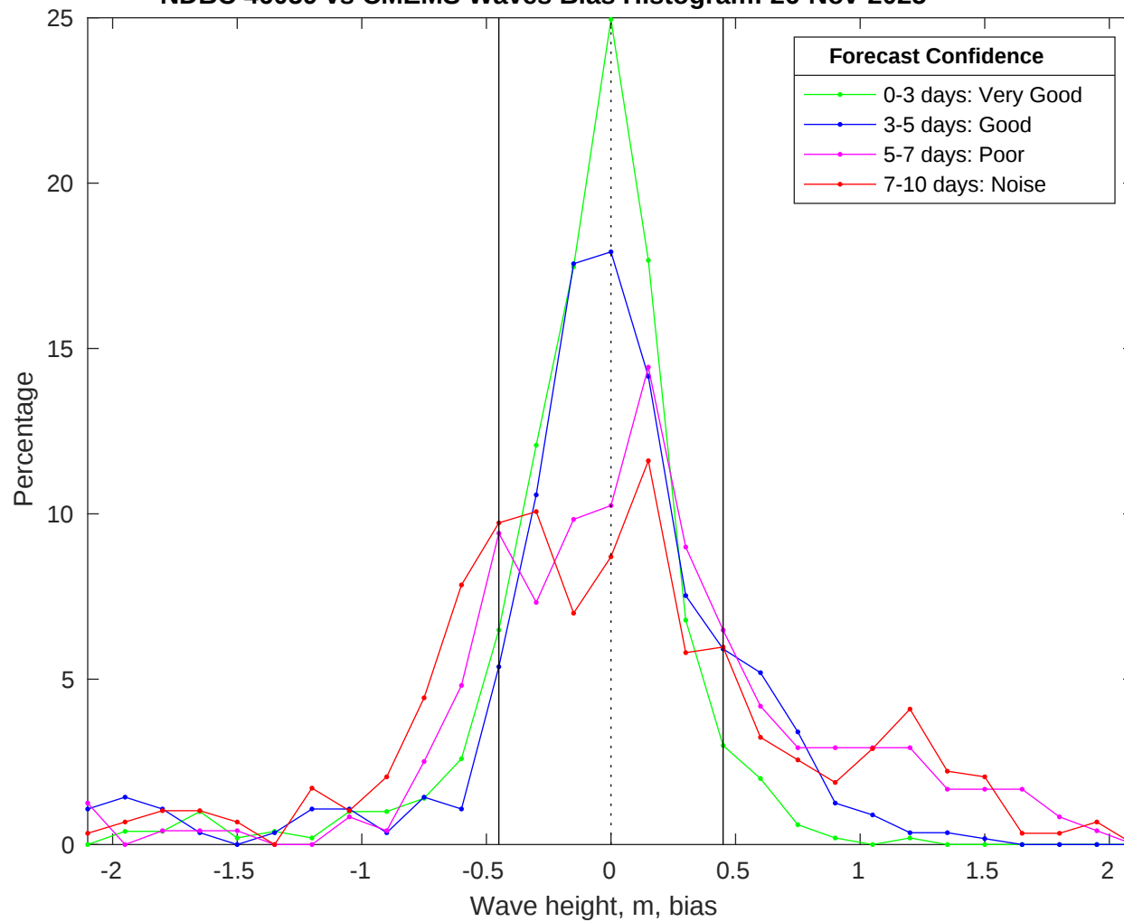
NDBC 46059 vs CMEMS Waves Bias Histogram: 26-Nov-2025
