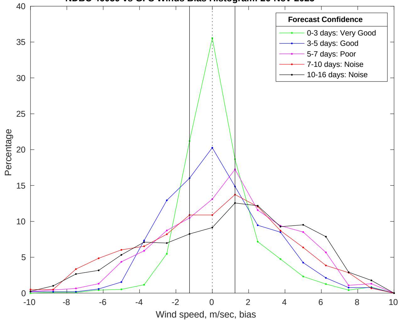
NDBC 46059 vs GFS Winds Bias Histogram: 26-Nov-2025
