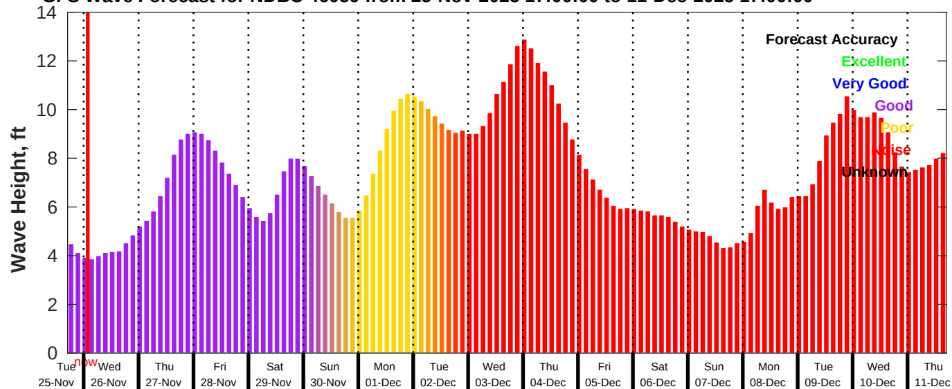
GFS Wave Forecast for NDBC 46059 from 25-Nov-2025 17:00:00 to 11-Dec-2025 17:00:00
