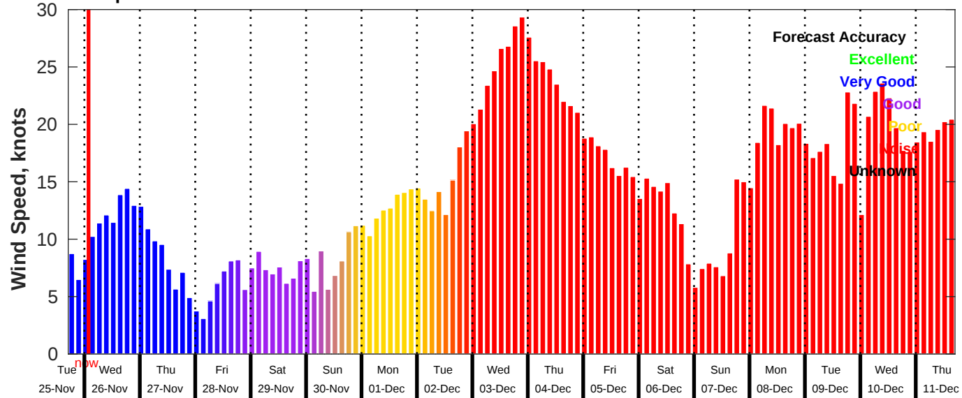
GFS Wind Speed Forecast for NDBC 46059 from 25-Nov-2025 17:00:00 to 11-Dec-2025 17:00:00
