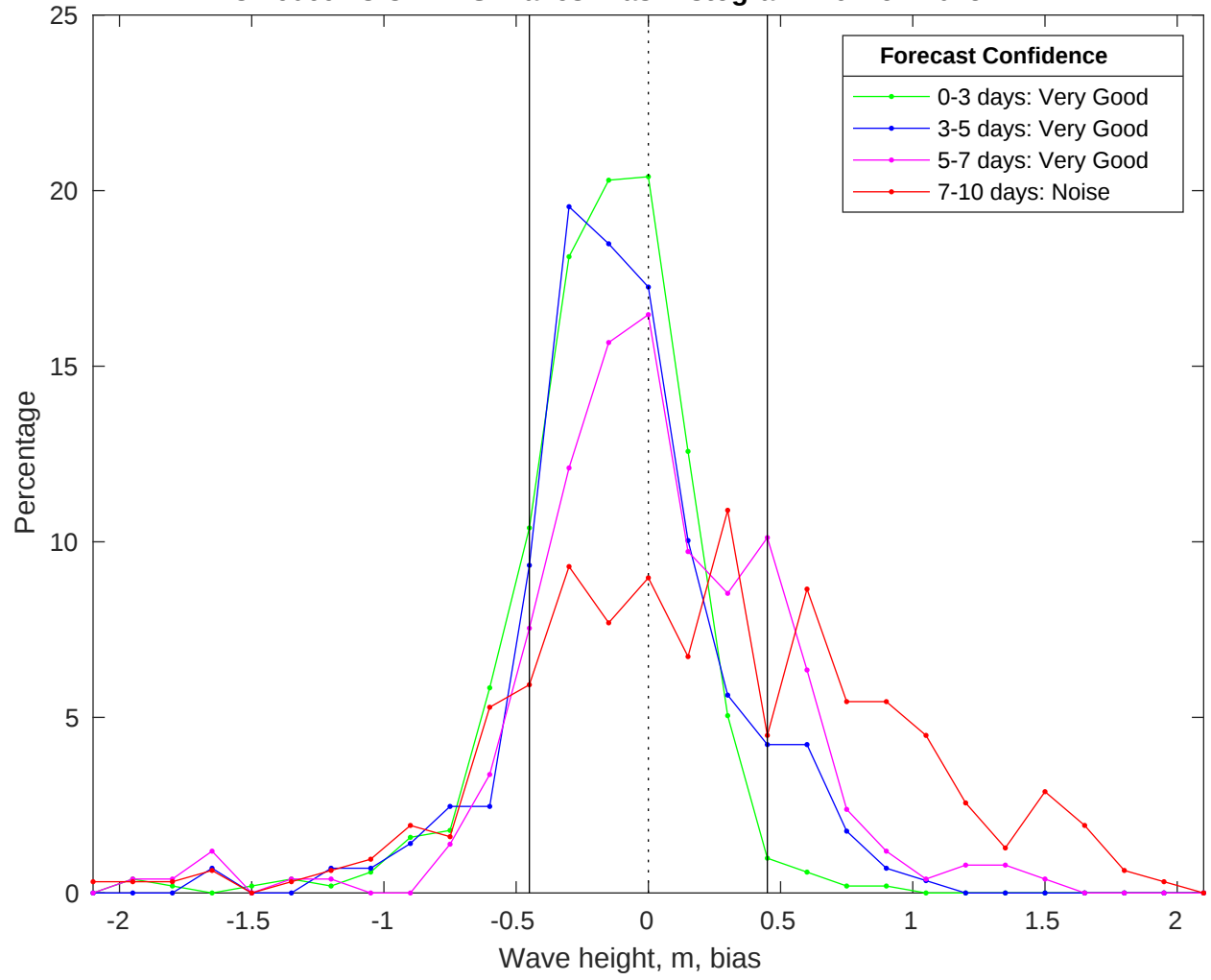
NDBC 46069 vs CMEMS Waves Bias Histogram: 26-Nov-2025
