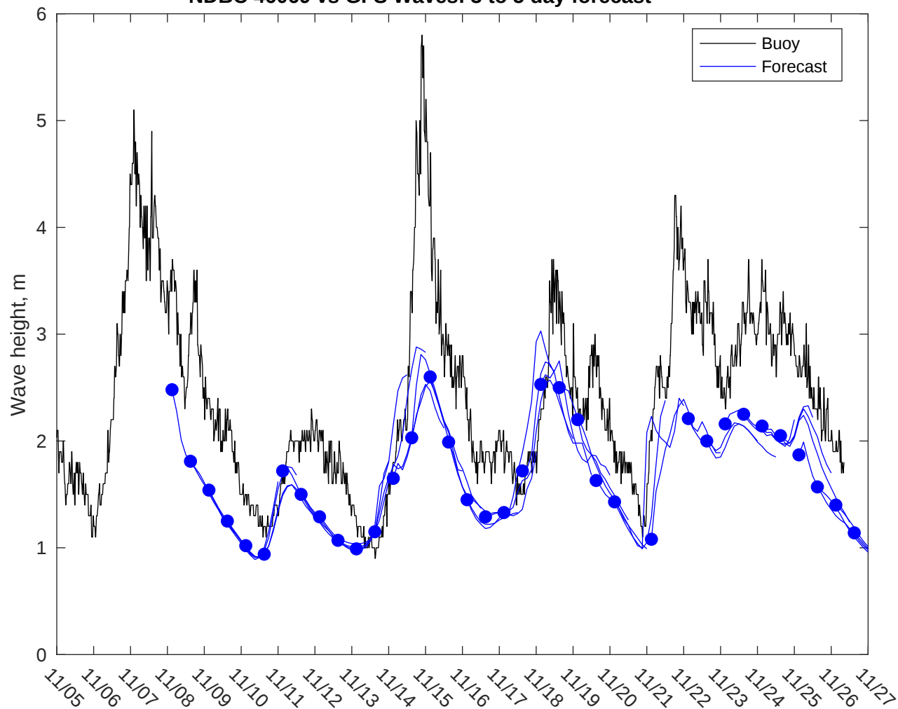
NDBC 46069 vs GFS Waves: 3 to 5 day forecast
