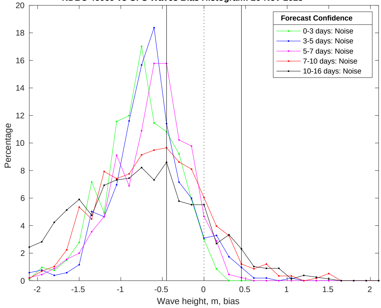
NDBC 46069 vs GFS Waves Bias Histogram: 26-Nov-2025
