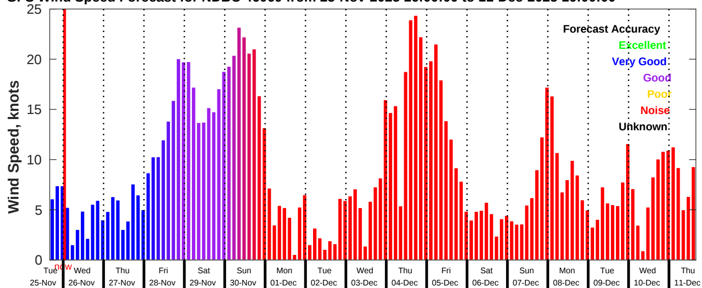
GFS Wind Speed Forecast for NDBC 46069 from 25-Nov-2025 16:00:00 to 11-Dec-2025 16:00:00
