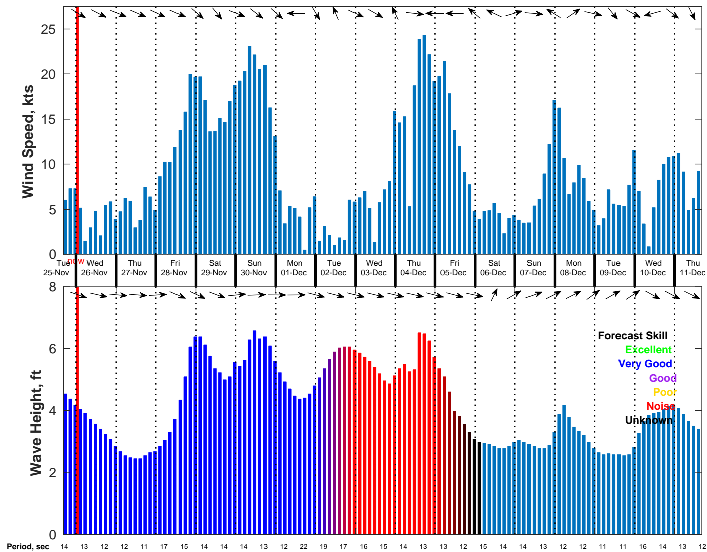
Wind & Wave Forecast for NDBC 46069 from 25-Nov-2025 16:00:00 to 11-Dec-2025 16:00:00
