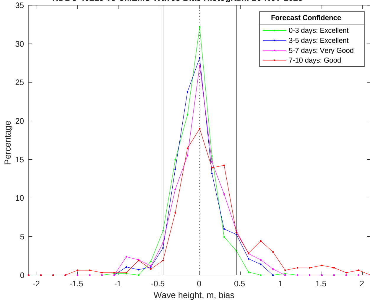
NDBC 46215 vs CMEMS Waves Bias Histogram: 26-Nov-2025
