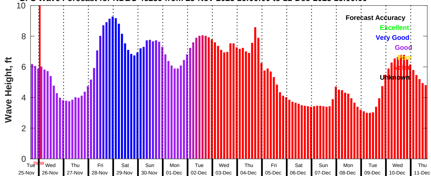
GFS Wave Forecast for NDBC 46259 from 25-Nov-2025 16:00:00 to 11-Dec-2025 16:00:00
