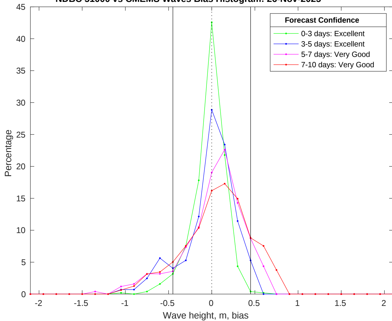
NDBC 51000 vs CMEMS Waves Bias Histogram: 26-Nov-2025
