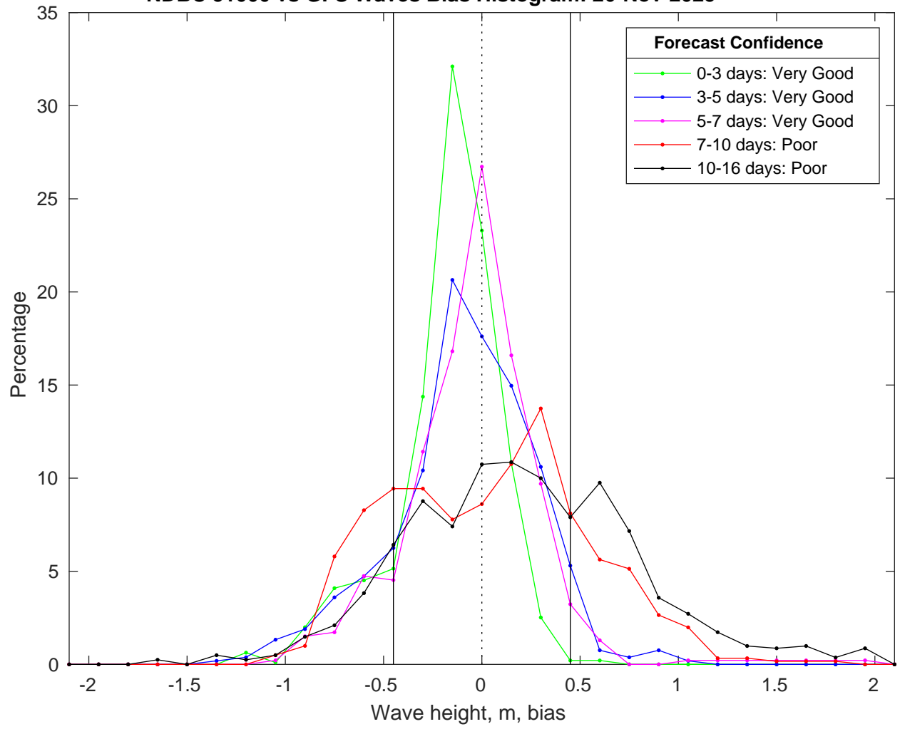
NDBC 51000 vs GFS Waves Bias Histogram: 26-Nov-2025
