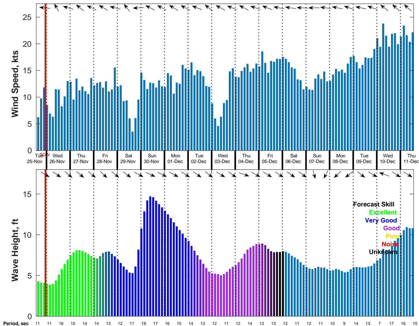
Wind & Wave Forecast for NDBC 51000 from 25-Nov-2025 14:00:00 to 11-Dec-2025 14:00:00
