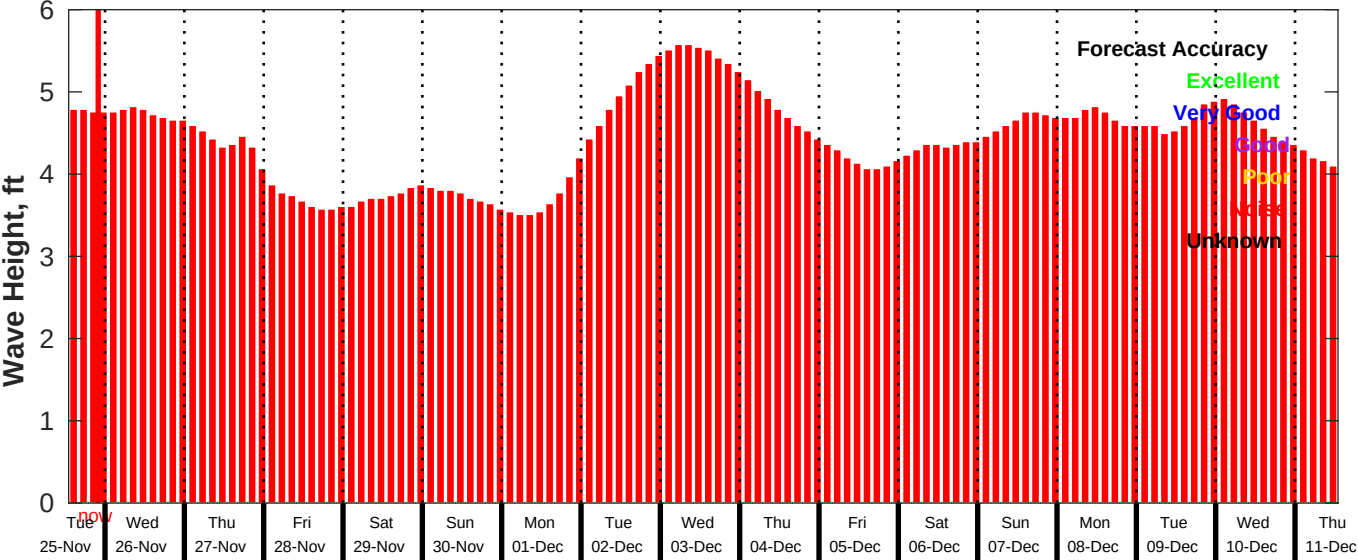
GFS Wave Forecast for NDBC 51209 from 25-Nov-2025 13:00:00 to 11-Dec-2025 13:00:00
