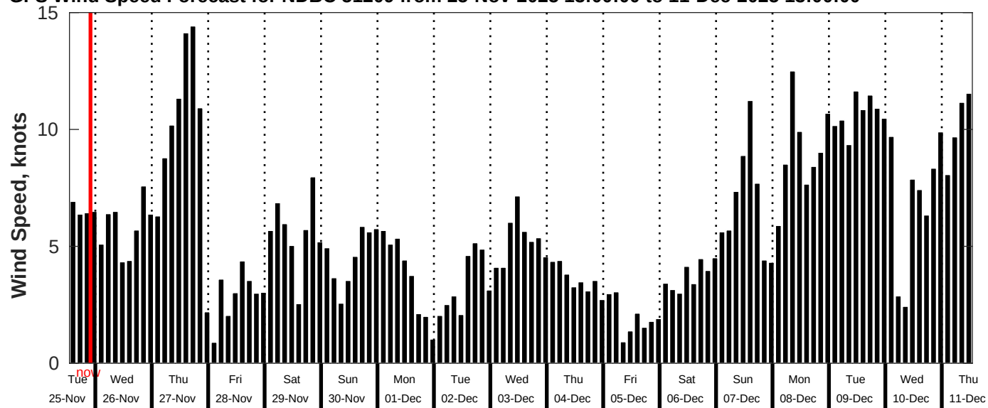
GFS Wind Speed Forecast for NDBC 51209 from 25-Nov-2025 13:00:00 to 11-Dec-2025 13:00:00
