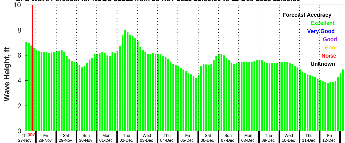
GFS Wave Forecast for NDBC 52211 from 26-Nov-2025 11:00:00 to 12-Dec-2025 11:00:00
