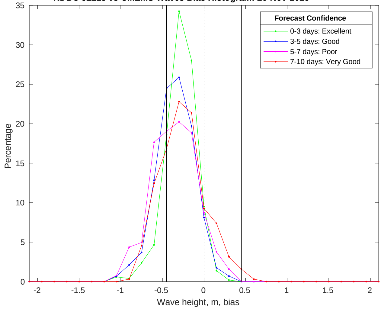
NDBC 52213 vs CMEMS Waves Bias Histogram: 26-Nov-2025
