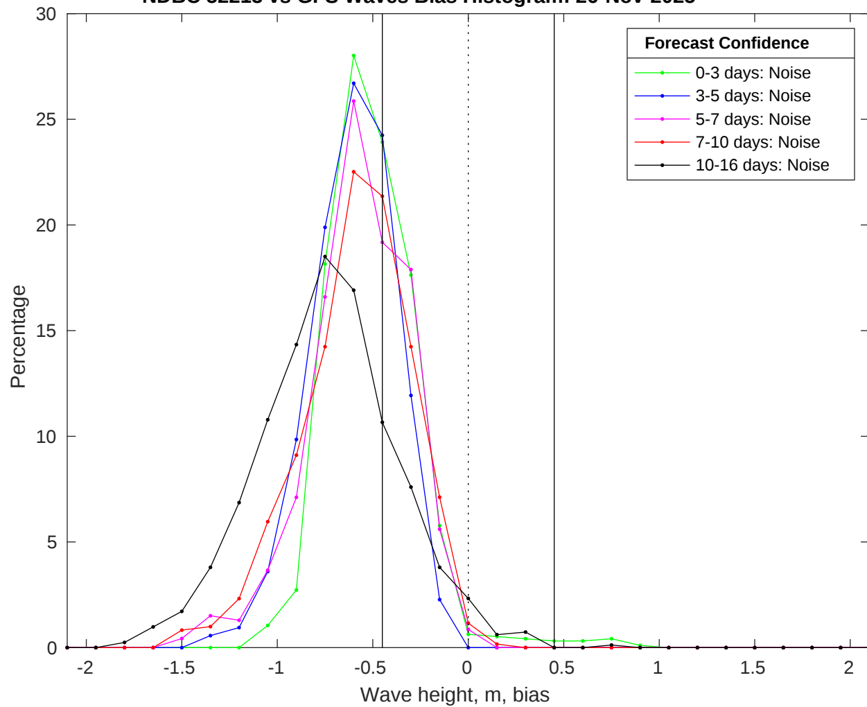
NDBC 52213 vs GFS Waves Bias Histogram: 26-Nov-2025
