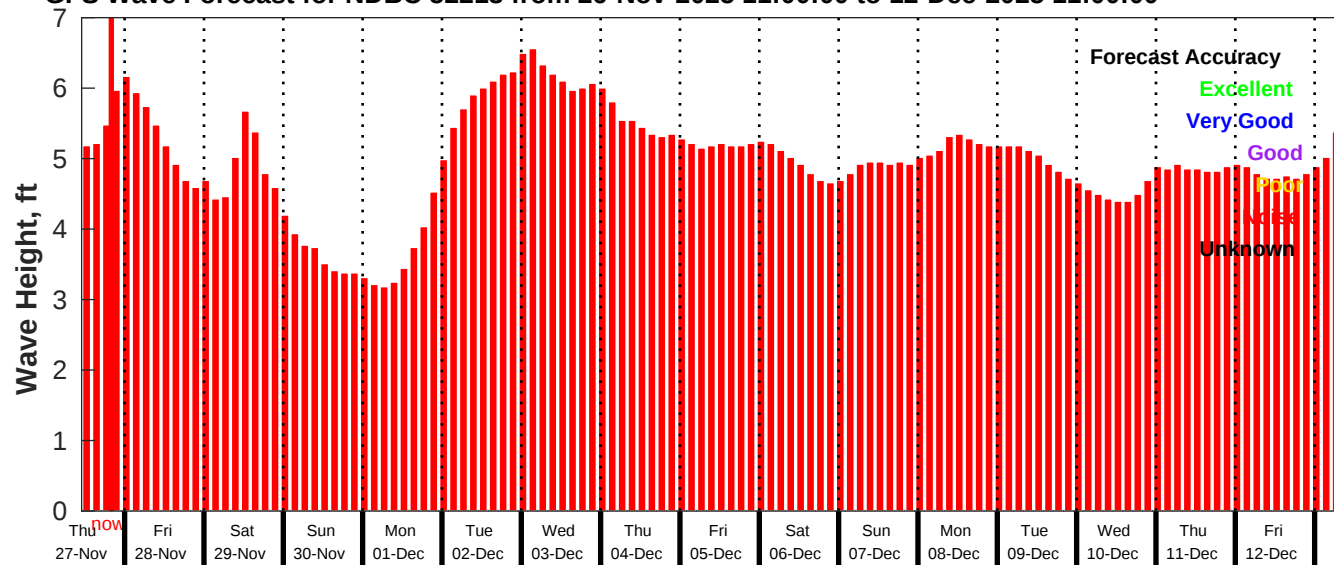
GFS Wave Forecast for NDBC 52213 from 26-Nov-2025 11:00:00 to 12-Dec-2025 11:00:00
