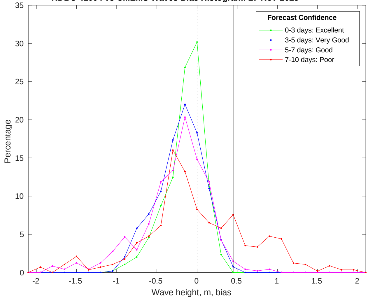
NDBC 41004 vs CMEMS Waves Bias Histogram: 27-Nov-2025
