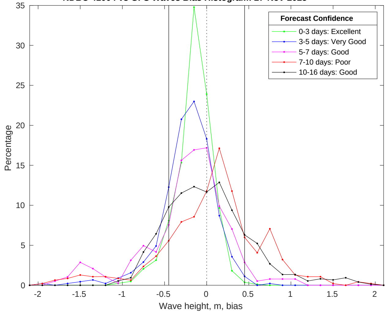
NDBC 41004 vs GFS Waves Bias Histogram: 27-Nov-2025
