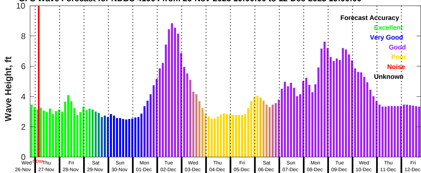
GFS Wave Forecast for NDBC 41004 from 26-Nov-2025 19:00:00 to 12-Dec-2025 19:00:00
