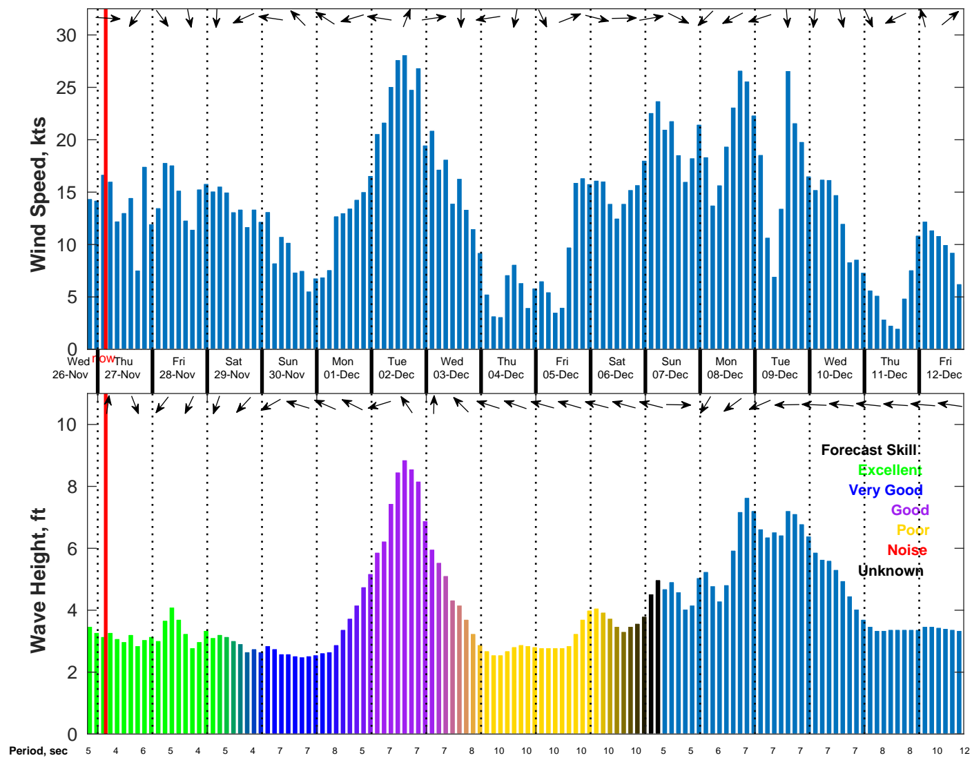
Wind & Wave Forecast for NDBC 41004 from 26-Nov-2025 19:00:00 to 12-Dec-2025 19:00:00
