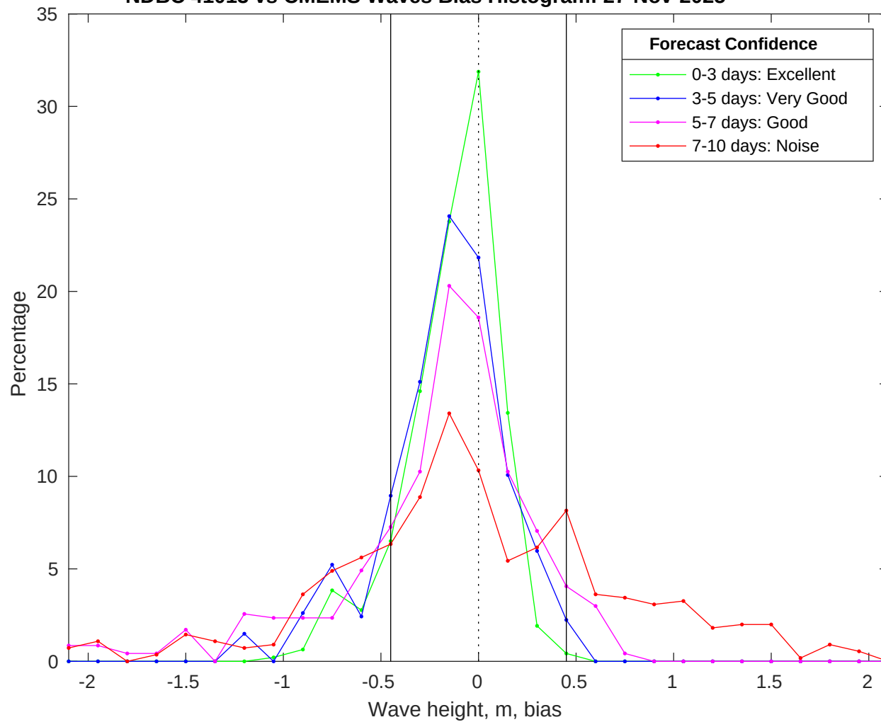
NDBC 41013 vs CMEMS Waves Bias Histogram: 27-Nov-2025
