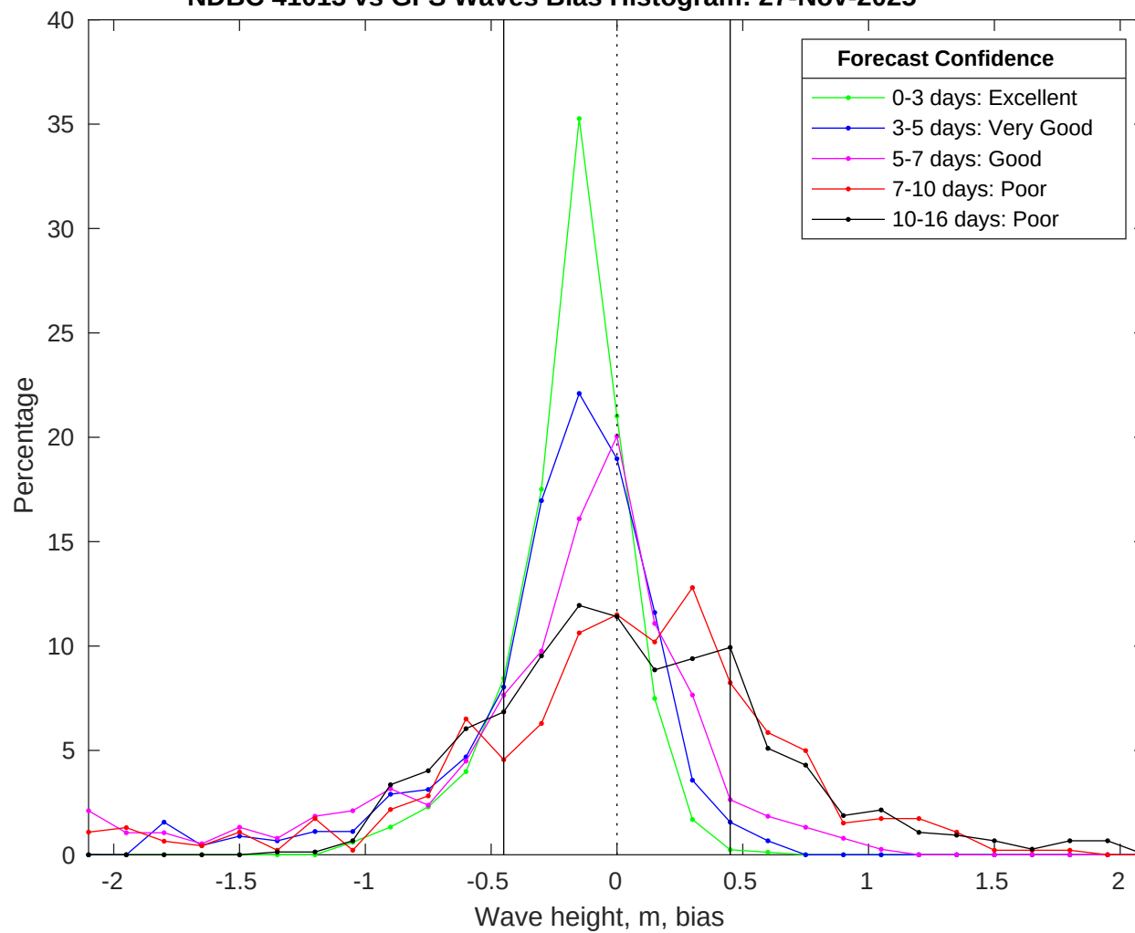
NDBC 41013 vs GFS Waves Bias Histogram: 27-Nov-2025
