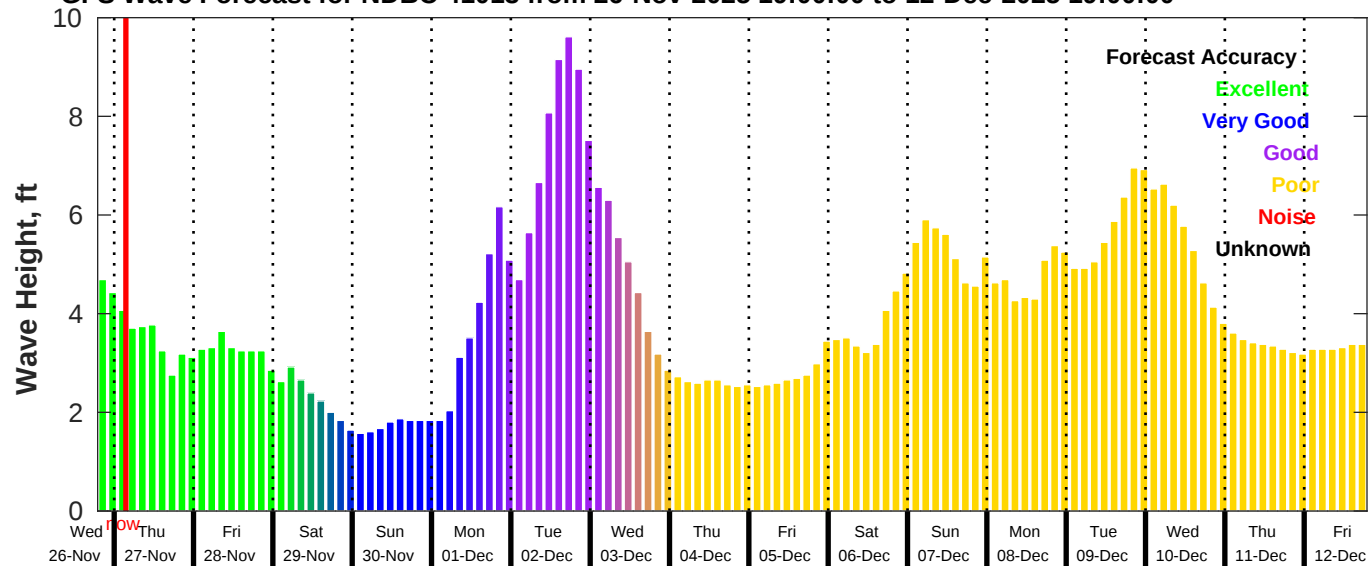
GFS Wave Forecast for NDBC 41013 from 26-Nov-2025 19:00:00 to 12-Dec-2025 19:00:00
