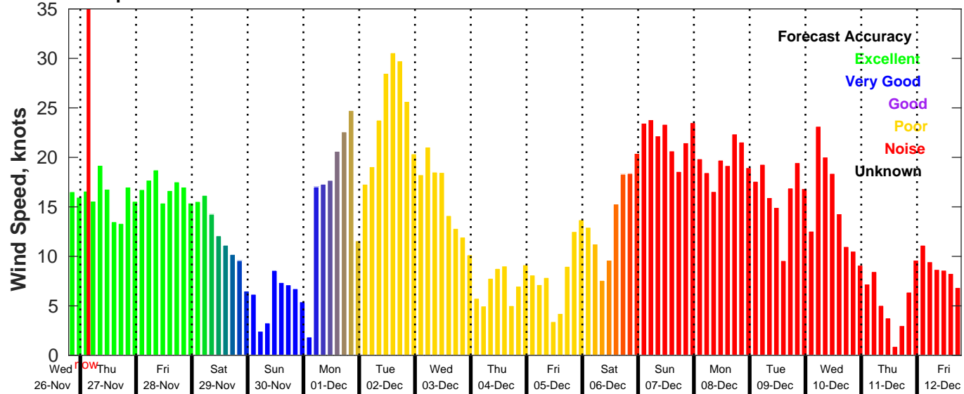
GFS Wind Speed Forecast for NDBC 41013 from 26-Nov-2025 19:00:00 to 12-Dec-2025 19:00:00
