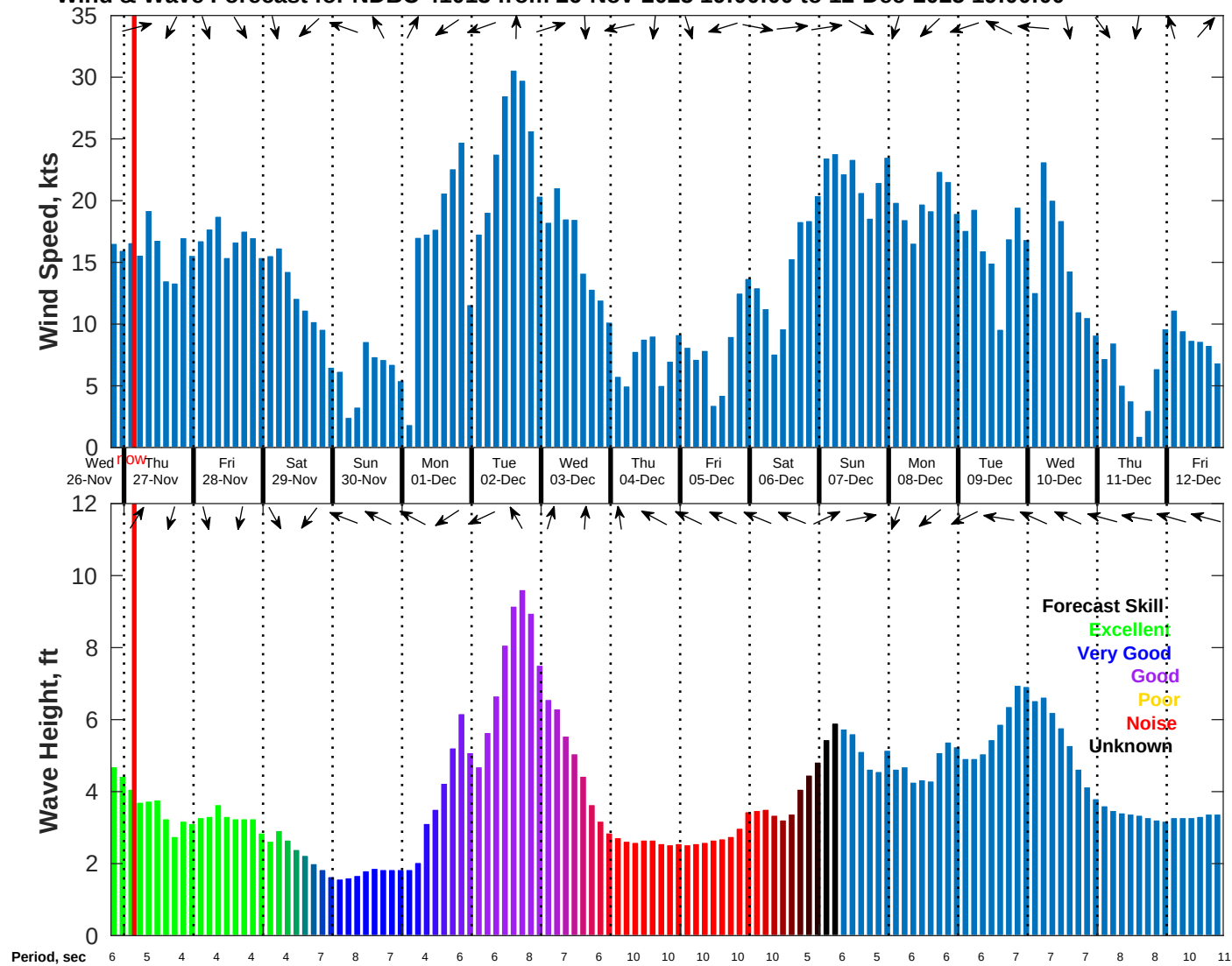
Wind & Wave Forecast for NDBC 41013 from 26-Nov-2025 19:00:00 to 12-Dec-2025 19:00:00
