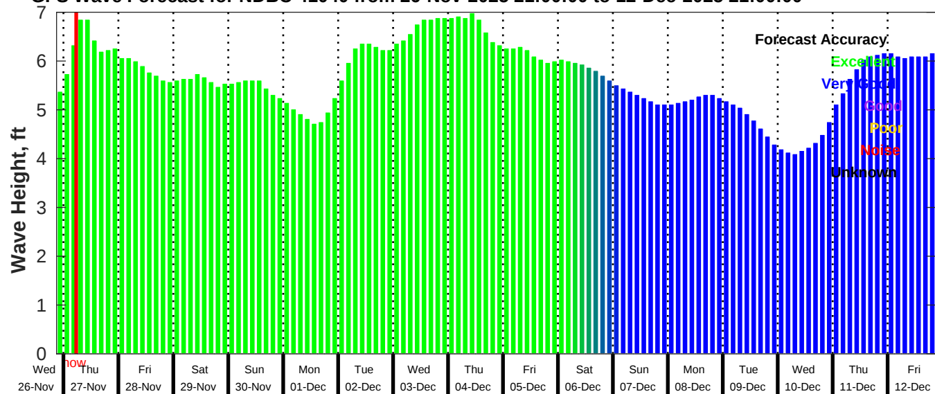
GFS Wave Forecast for NDBC 41040 from 26-Nov-2025 21:00:00 to 12-Dec-2025 21:00:00
