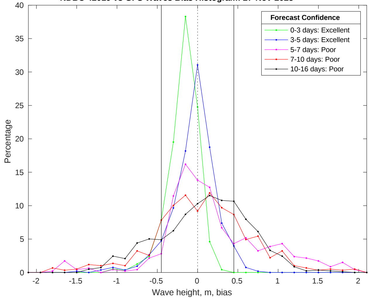
NDBC 42019 vs GFS Waves Bias Histogram: 27-Nov-2025
