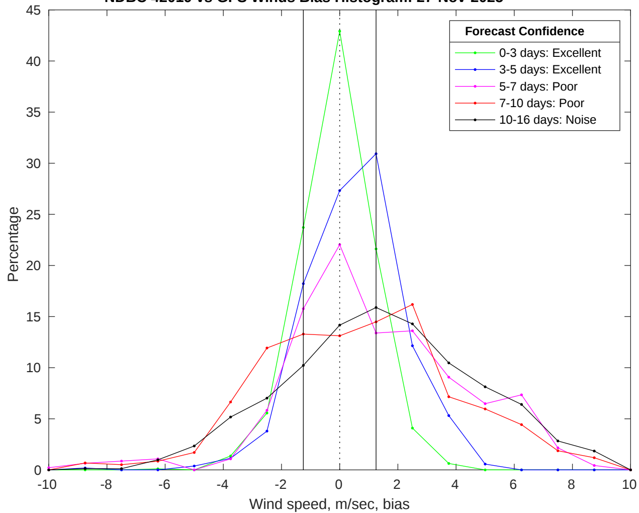
NDBC 42019 vs GFS Winds Bias Histogram: 27-Nov-2025
