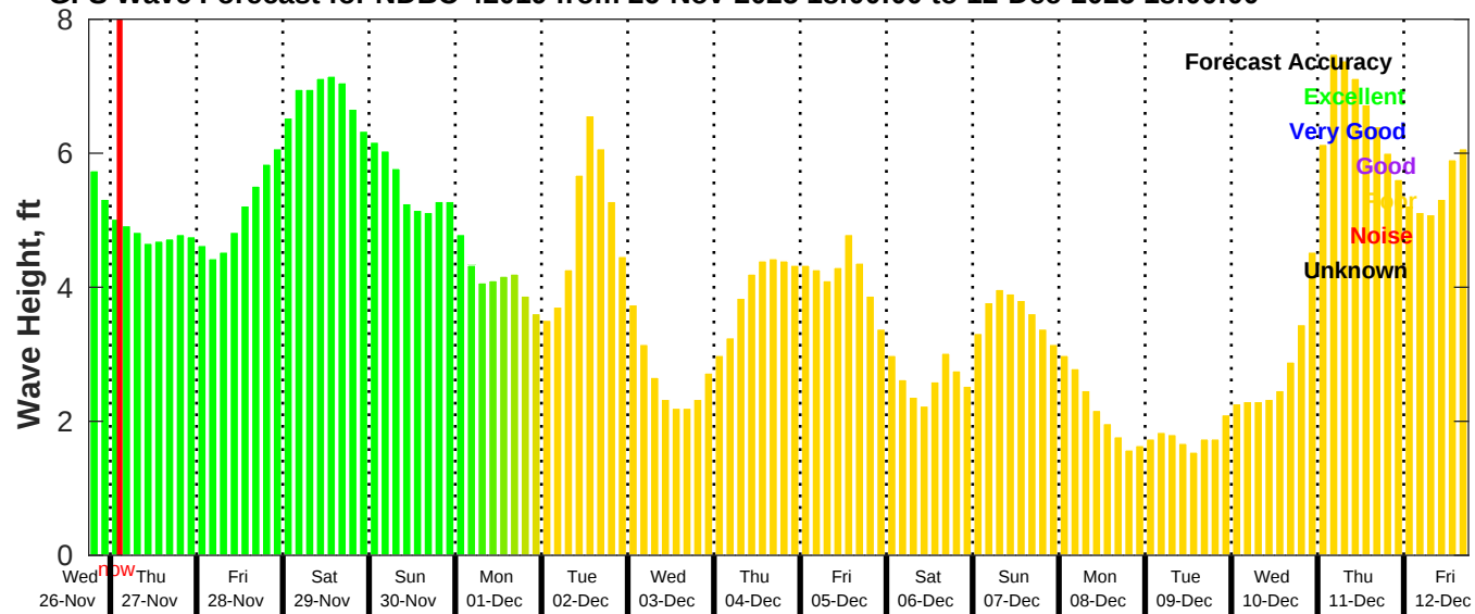
GFS Wave Forecast for NDBC 42019 from 26-Nov-2025 18:00:00 to 12-Dec-2025 18:00:00
