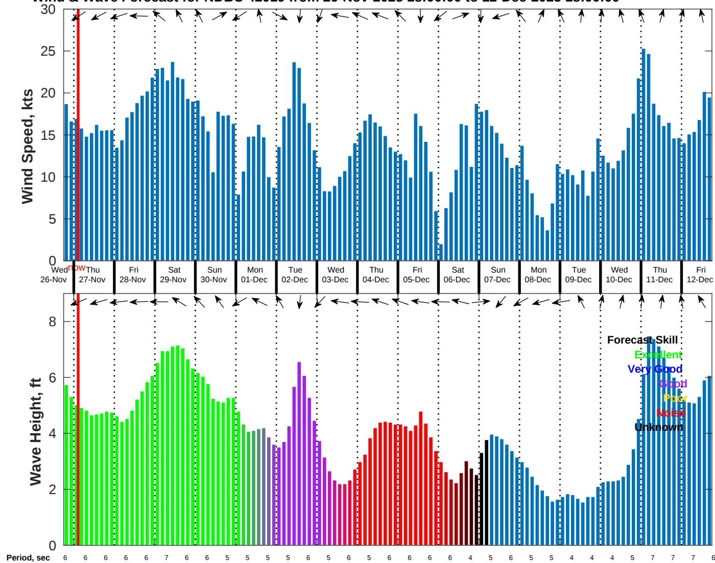
Wind & Wave Forecast for NDBC 42019 from 26-Nov-2025 18:00:00 to 12-Dec-2025 18:00:00
