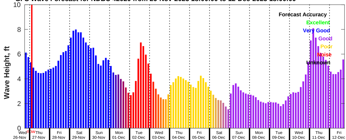
GFS Wave Forecast for NDBC 42020 from 26-Nov-2025 18:00:00 to 12-Dec-2025 18:00:00
